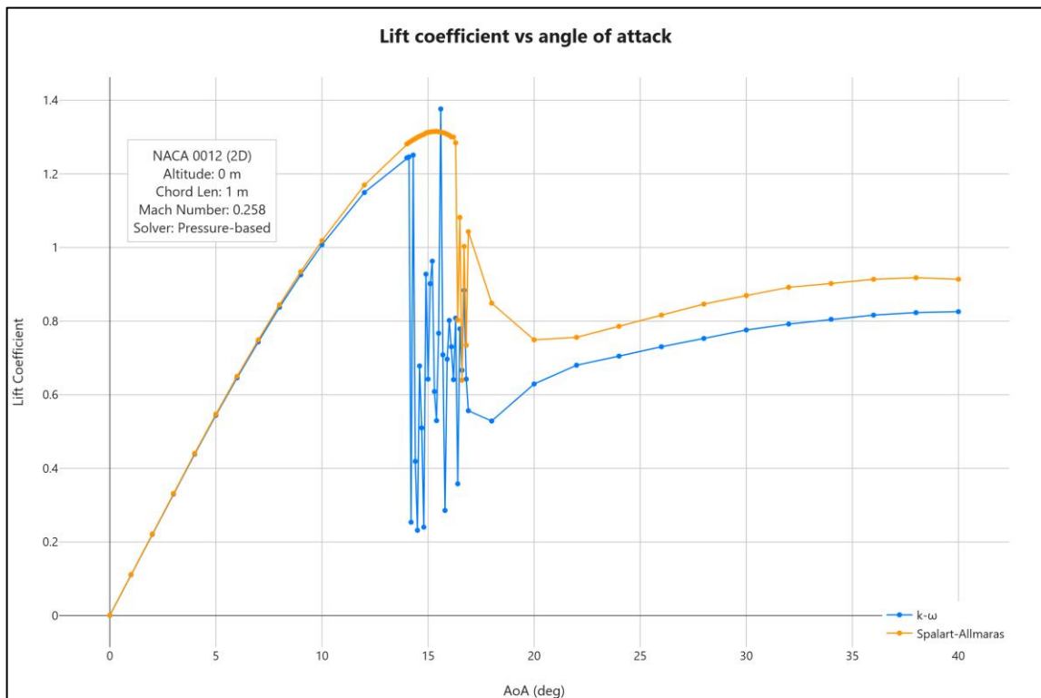
Figure 4-64 - Lift coefficient at different angles of attack
