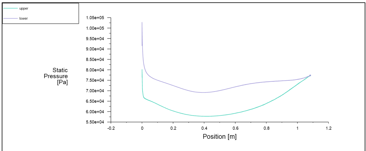
Figure 4-11 - Pressure plot of the optimised NACA 0012 design (variable length)
