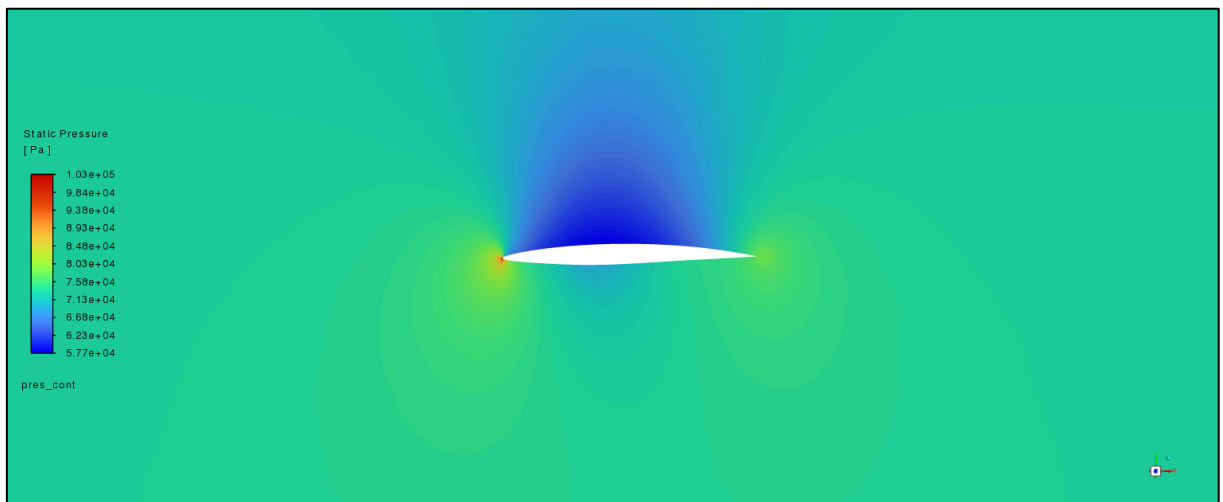
Figure 4-9 - Pressure contours of the optimised NACA 0012 design (variable length)
