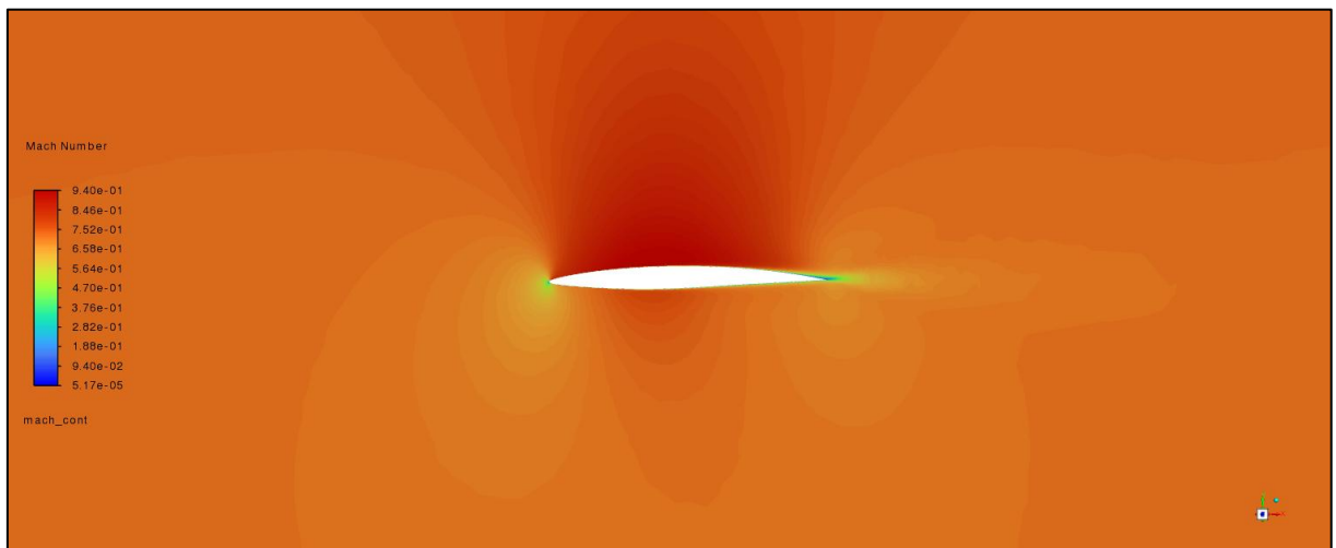
Figure 4-7 - Mach contours of the optimised NACA 0012 design (variable length)
