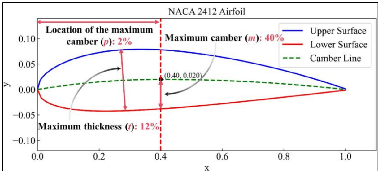
Figure 2-7 - NACA 2412 Airfoil [14]
