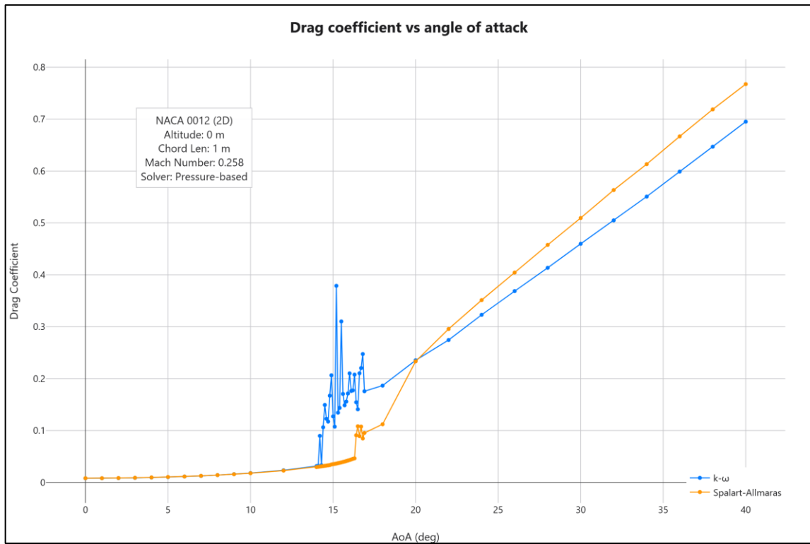
Figure 4-63 - Drag coefficient at different angles of attack
