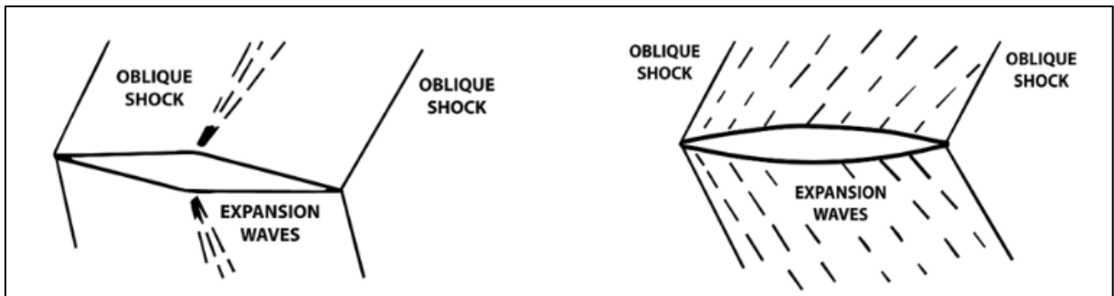
Figure 2-9 - A visualisation of supersonic airflow over a double-wedge airfoil (left) and biconvex airfoil (right) [19]
